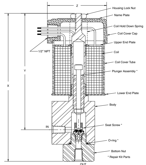
2004 Series 1/8" valve shown with NEMA 1 coil housing and a soft seat
