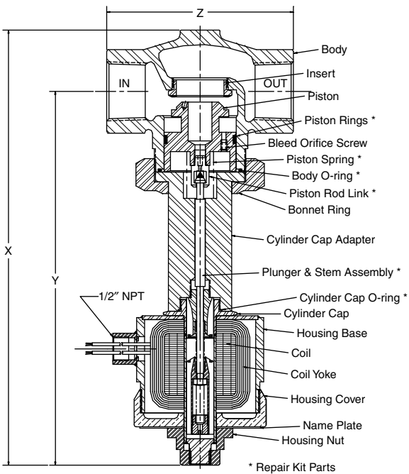
Normally open 1 1/2" 42861 valve, shown with a NEMA 7 explosion-proof coil housing and a AC coil
